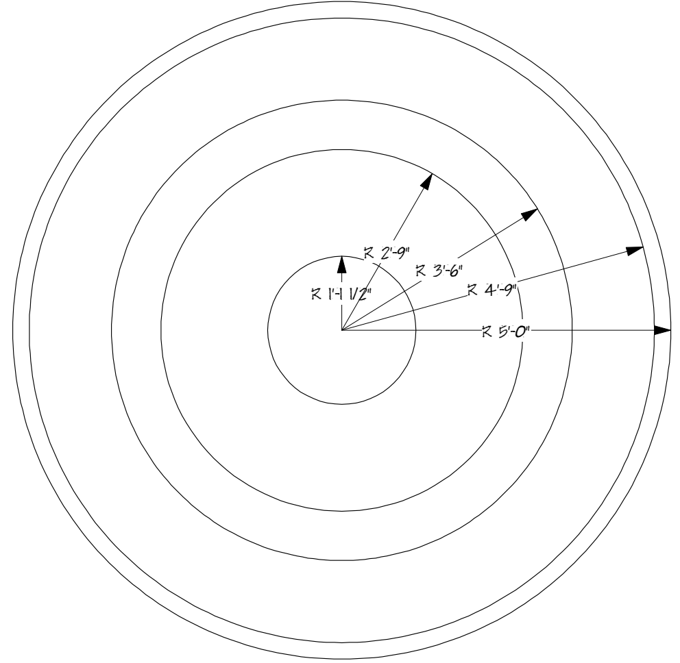
2 SMALL PLATFORM LAYOUT SCALE: 1/2" = 1'-0"
